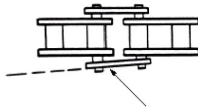
FIGURE 3 - Link Plate Distortion
