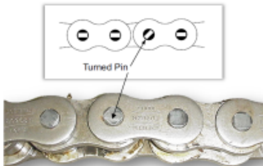
FIGURE 2 - Turned Pin
